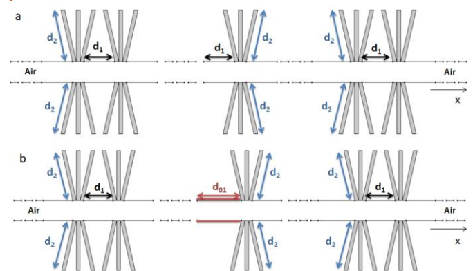
Figure: (a) One-dimensional star waveguide phononic structure containing N period (cellule), each period contains by the segment of length d_1 and grafted in each site by one resonator of height d_2 . (b) Same as (a) except that there is a segment defect of the length d_{01} located in the center of the periodic structure
