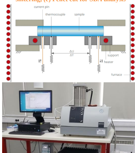
Figure 2. Measurement setup of the SBA 458 Nemesis
