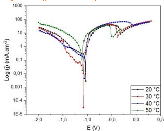
Figures: Polarization measurements of electrodeposited coatings with different bath temperatures in 3.5% NaCl
