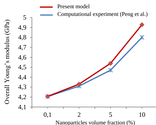
Figure 2: Overall Young's modulus of nanocomposite as a function of nanoparticle volume fraction (interphase thickness = 0.6nm)
