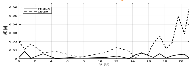
Fig.2 Individual absolute error (IAE) between experimental and simulated I(V) curves using the five parameters extracted by TRDLA or LSQM.
