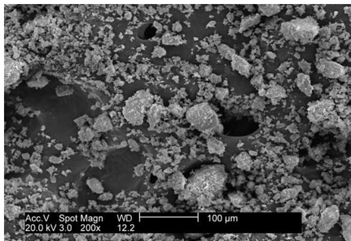
Figure: Typical topographic image for the material by Scanning Electron Photomicrographs (SEM). Bar length is 100µm and the magnification 200x
