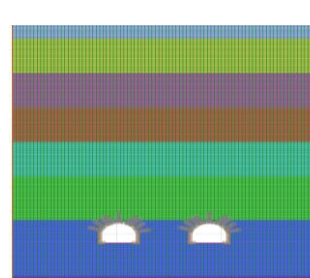
Figure 1: Constitutive model of cross section 1
