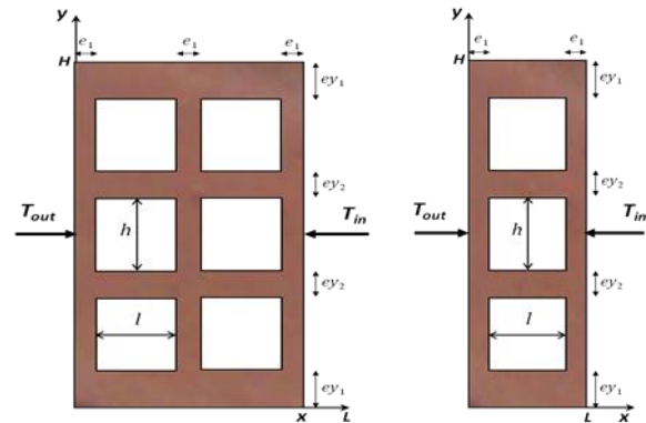
Figures: Studied hollow clay bricks
