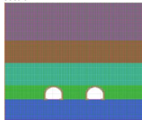
Figure 1: Constitutive model of cross section 1
