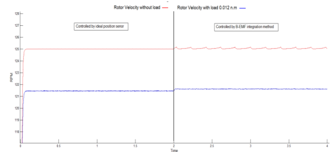
Figure 2 Rotor Velocity with and without load
