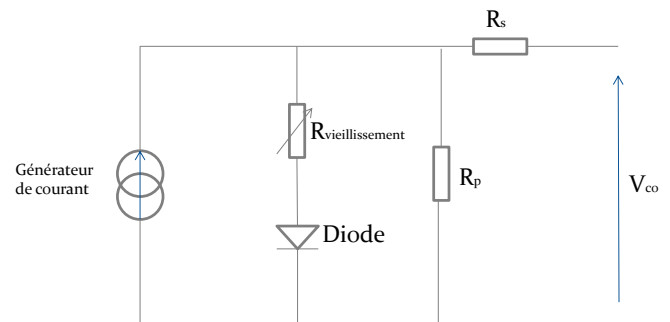
Figure: Model of a degraded photovoltaic cell
