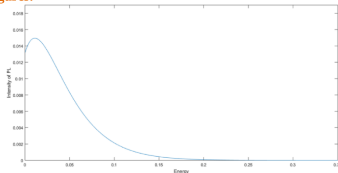
Fig. 1. Photoluminescence spectrum of a InAs/GaAs QDs at T = 77 K
