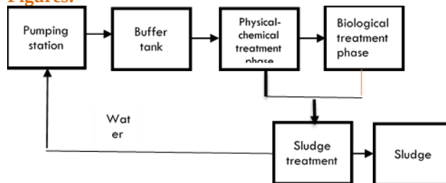
Figure 1: Diagram of process of WWTP
