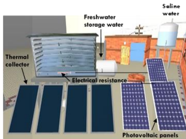
Figure: synoptic diagrams of MSDH hybrid still
