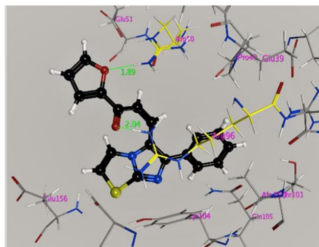
Figure: 3D interactions of one of the compounds into the binding site of P. aeruginosa Thymidylate kinase
