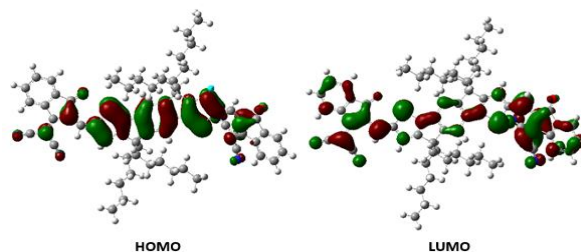
Figure 5: The contour plots of HOMO and LUMO orbitals of the IDIC compound.
