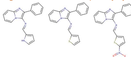
Figure: Chemical structure for the proposed compounds
