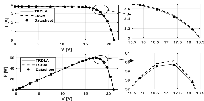
Fig.1 Experimental current-voltage I(V) and power-voltage P(V) characteristics of poly-crystalline (MSX60) silicon PV panel at STC compared to the calculated data by taking account of the five parameters obtained by TRDLA and LSQM.
