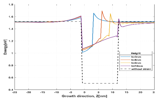
Fig.1. The conduction band with strain effect (solid line) for different heights and without strain effect in a QD structure with a height of 12 nm.
