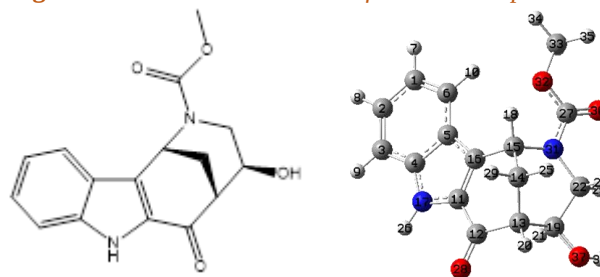
Figure: The chemical structure of the title compound
