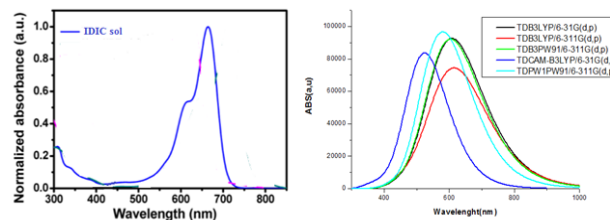
Figure 4: Experimental absorption in the UV-visible of IDIC compound in dichloromethane solution ( 10^{-5} M) (on the left); absorption spectra in UV-visible of IDIC compound simulated by the TD-DFT level with different functions in gaseous state (on the right).
