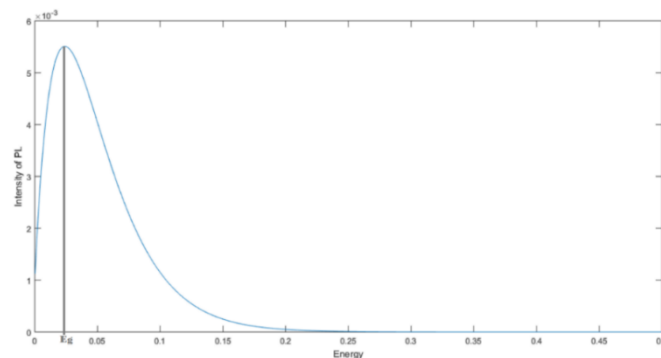
Fig. 2. Photoluminescence spectrum of a InAs/GaAs QDs at T = 300 K
