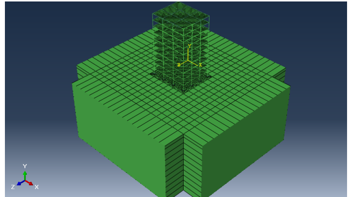
Figure: Abaqus CA Model with Infinte Soil Element
