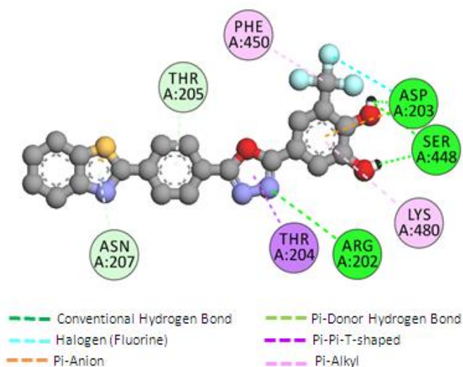
Figure: Docking interactions of the proposed compound X1
