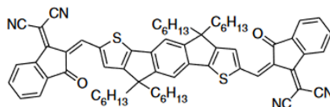
Figure 1: Chemical structure of the IDIC compound
