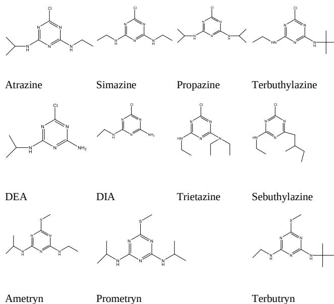
Figure: Chemical structures of the studied compounds
