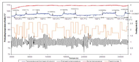
Fig. Normal behavior of rectification column.
