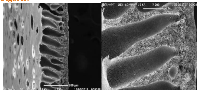
SEM micrographs of cross-section PSU/PVP/TREN membrane
