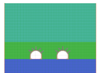
Figure 2 : Constitutive model of cross section 2
