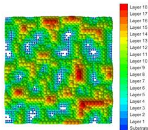
Figure: Top view of the deposited CdTe/(001)GaAs film (14.7% lattice mismatch)
